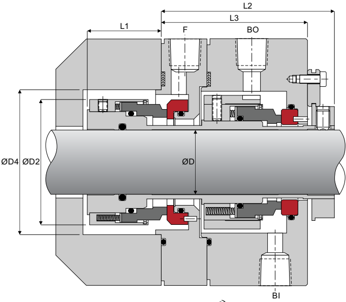
Optional Medium Pressure Design
